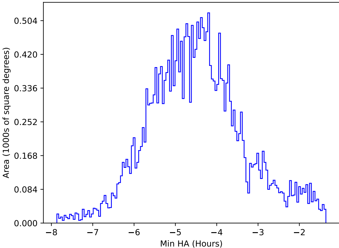
internal_u_expt60_nscale1.0v3.4_10yrs All sky all bands: Min HA
