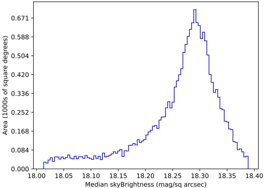
internal_u_expt60_nscale1.0v3.4_10yrs WFD y band: Median skyBrightness
