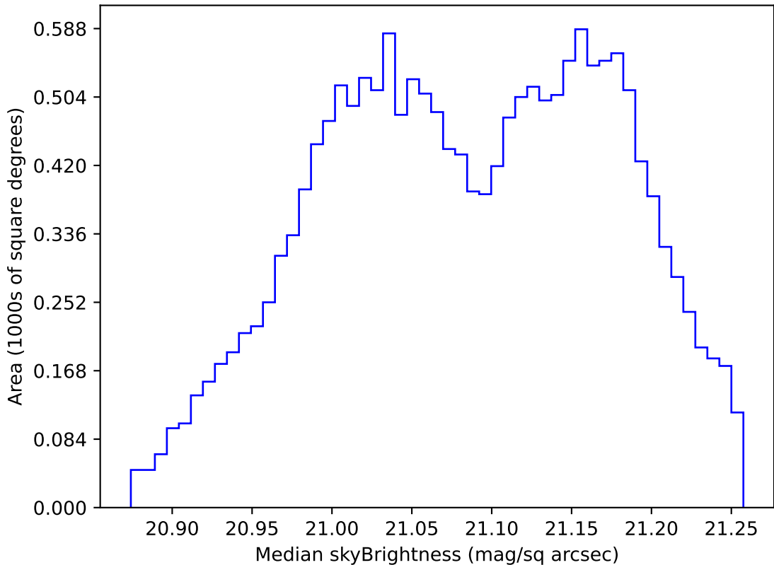
internal_u_expt60_nscale1.0v3.4_10yrs WFD r band: Median skyBrightness
