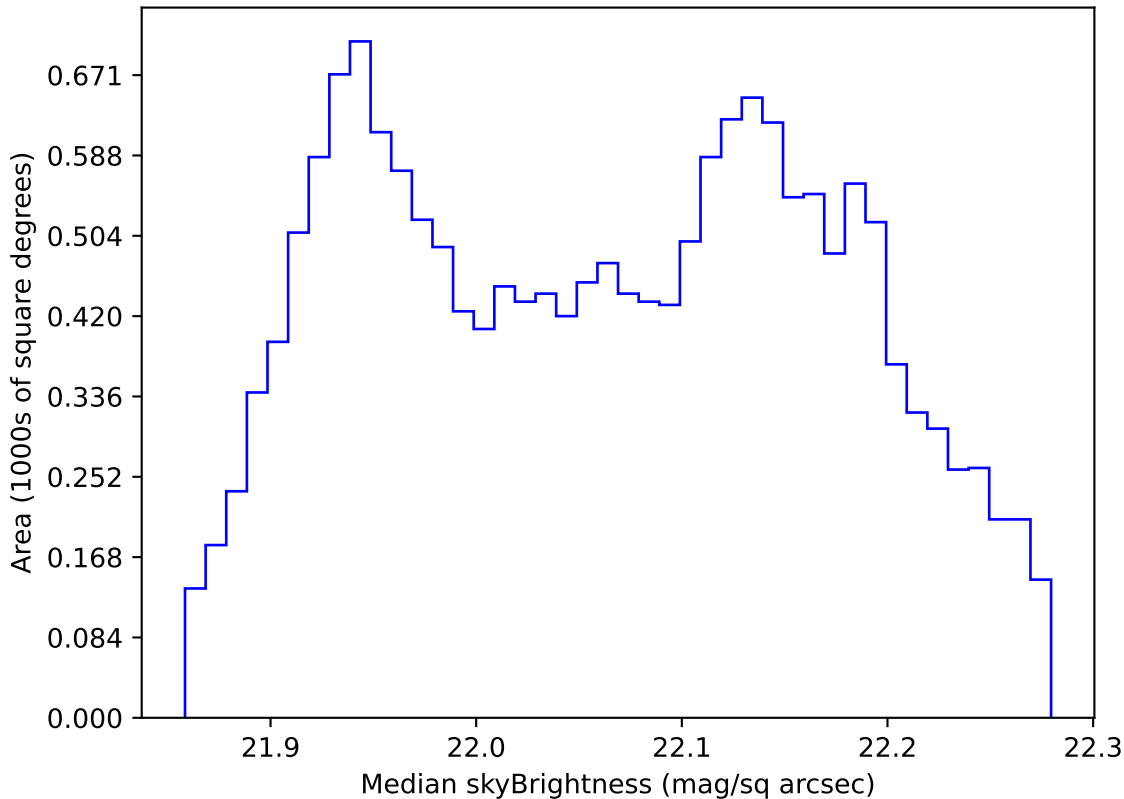
internal_u_expt60_nscale1.0v3.4_10yrs WFD g band: Median skyBrightness
