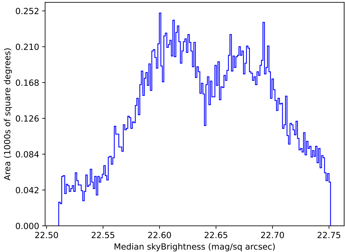
internal_u_expt60_nscale1.0v3.4_10yrs All sky u band: Median skyBrightness
