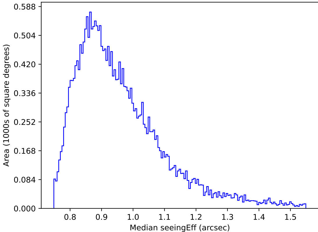
internal_u_expt60_nscale1.0v3.4_10yrs Yr 1 i band: Median seeingEff
