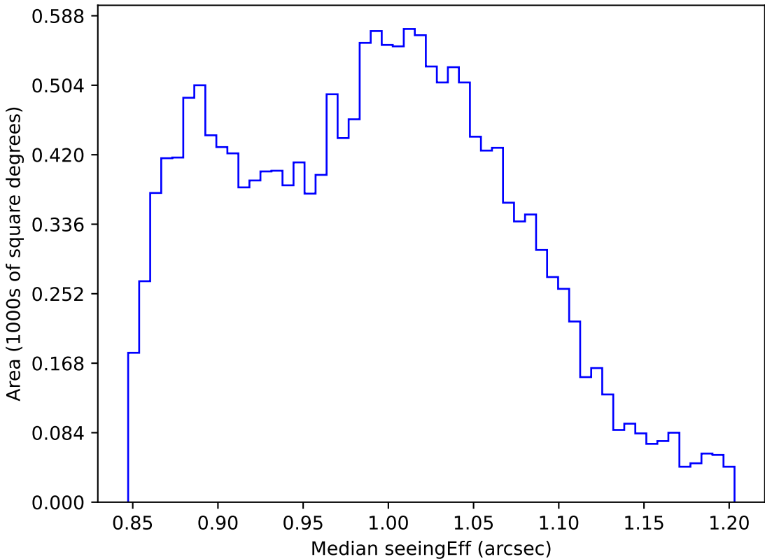
internal_u_expt60_nscale1.0v3.4_10yrs WFD i band: Median seeingEff
