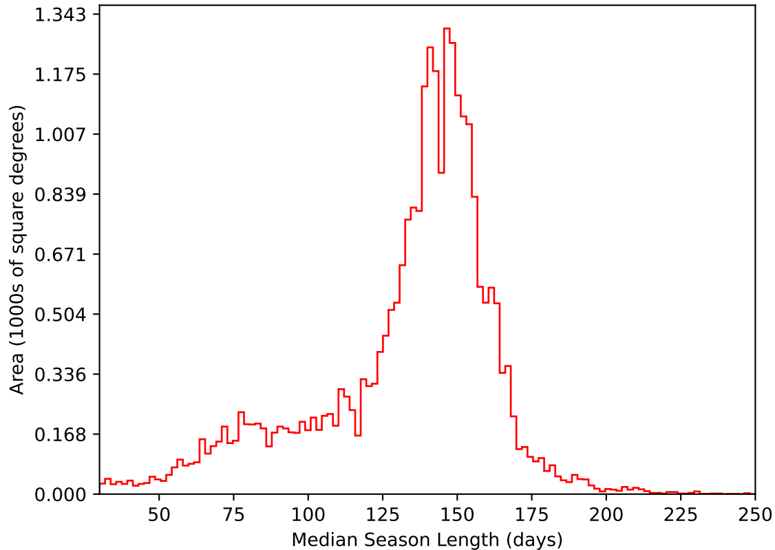
internal_u_expt60_nscale1.0v3.4_10yrs All sky i band: Median Season Length
