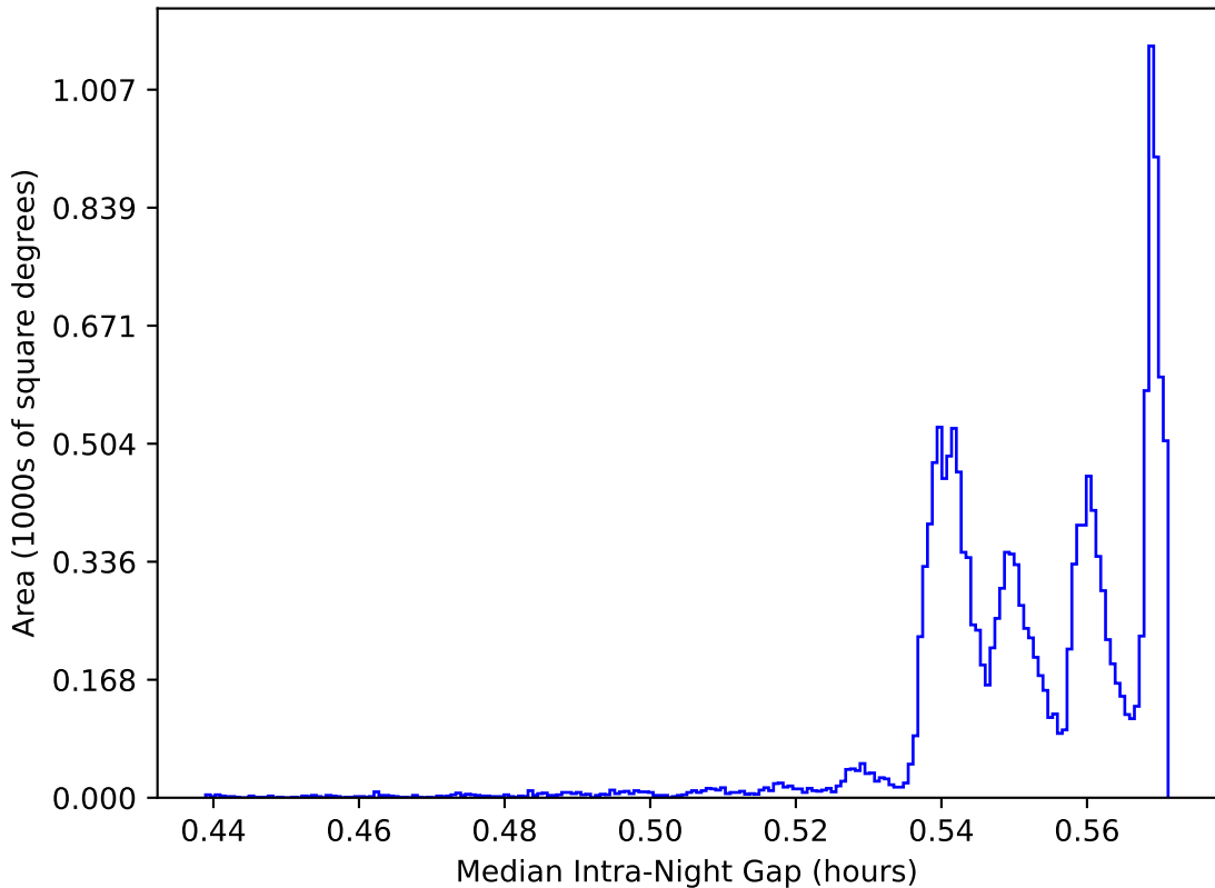
internal_u_expt60_nscale1.0v3.4_10yrs WFD: Median Intra-Night Gap
