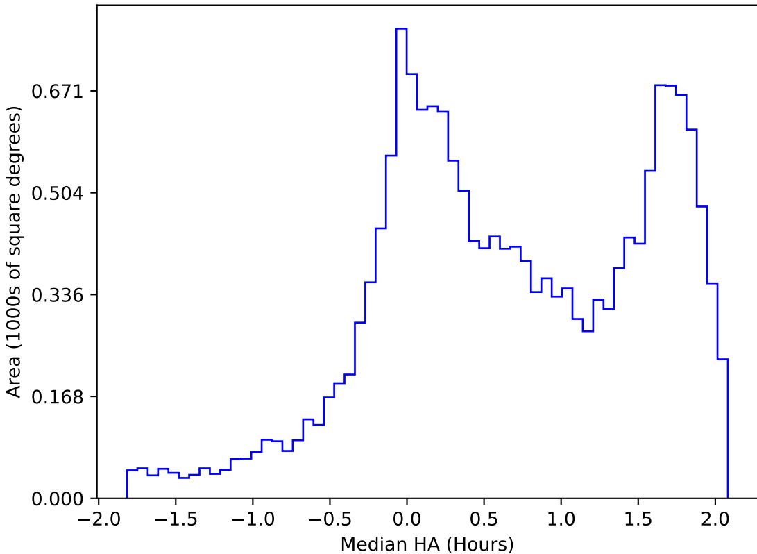
internal_u_expt60_nscale1.0v3.4_10yrs WFD g band: Median HA
