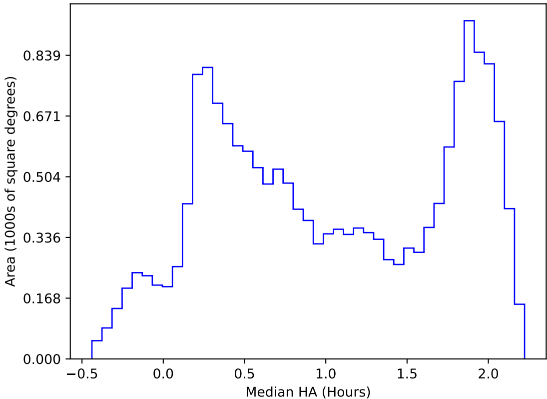
internal_u_expt60_nscale1.0v3.4_10yrs WFD all bands: Median HA
