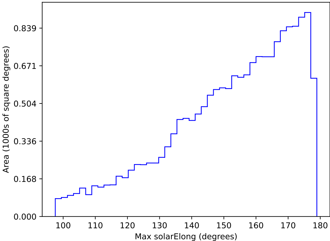
internal_u_expt60_nscale1.0v3.4_10yrs WFD u band: Max solarElong
