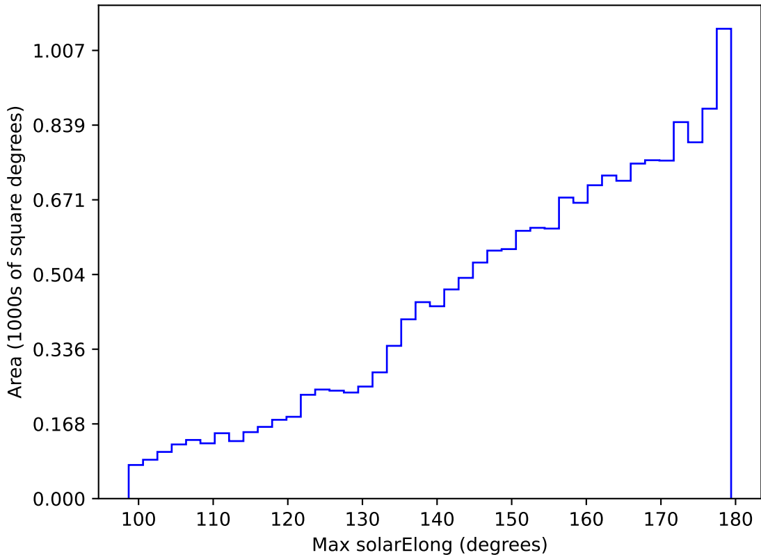
internal_u_expt60_nscale1.0v3.4_10yrs WFD r band: Max solarElong
