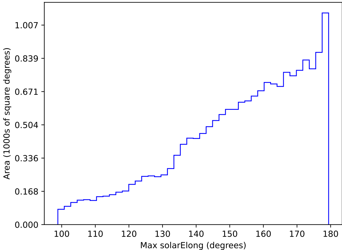
internal_u_expt60_nscale1.0v3.4_10yrs WFD i band: Max solarElong
