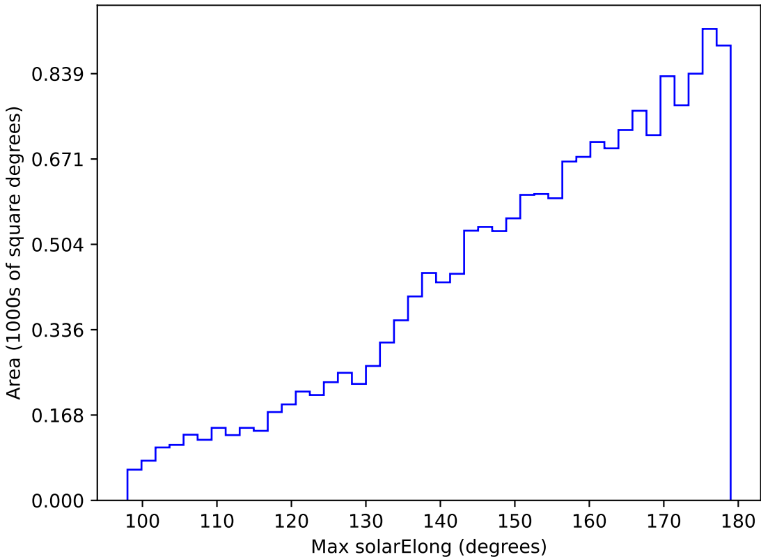
internal_u_expt60_nscale1.0v3.4_10yrs WFD g band: Max solarElong
