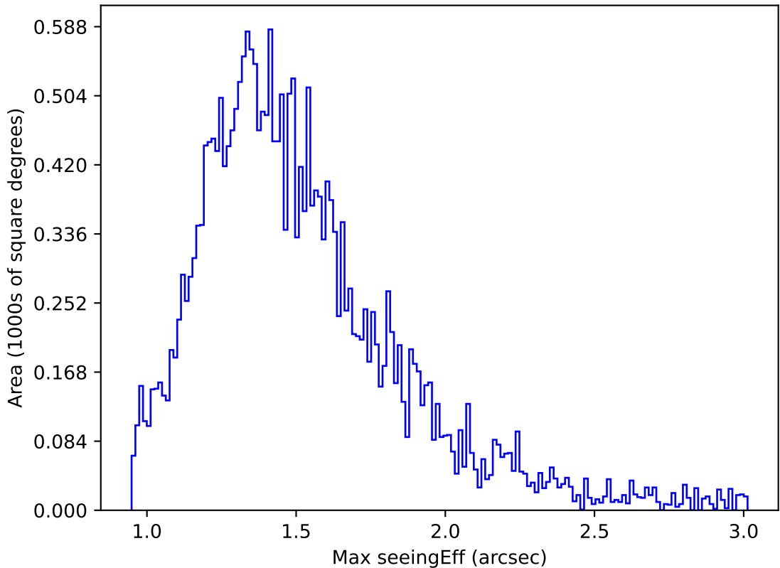
internal_u_expt60_nscale1.0v3.4_10yrs Yr 1 z band: Max seeingEff
