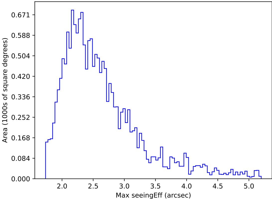
internal_u_expt60_nscale1.0v3.4_10yrs WFD z band: Max seeingEff
