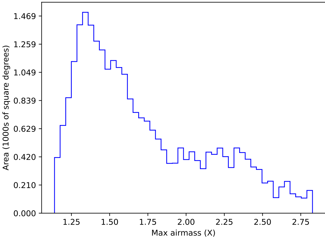
internal_u_expt60_nscale1.0v3.4_10yrs Yr 1 z band: Max airmass
