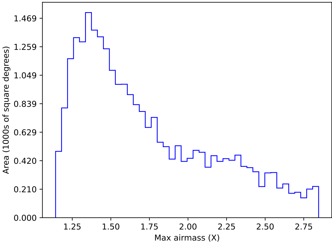
internal_u_expt60_nscale1.0v3.4_10yrs Yr 1 i band: Max airmass
