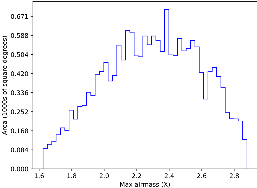
internal_u_expt60_nscale1.0v3.4_10yrs WFD y band: Max airmass
