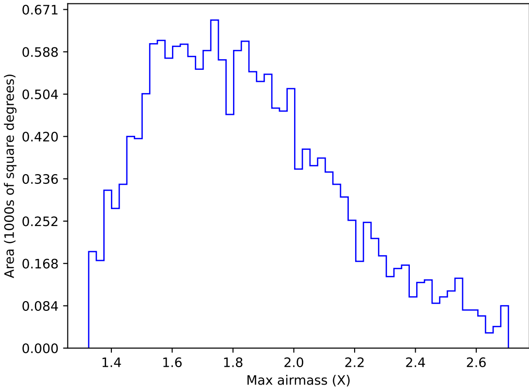
internal_u_expt60_nscale1.0v3.4_10yrs WFD u band: Max airmass
