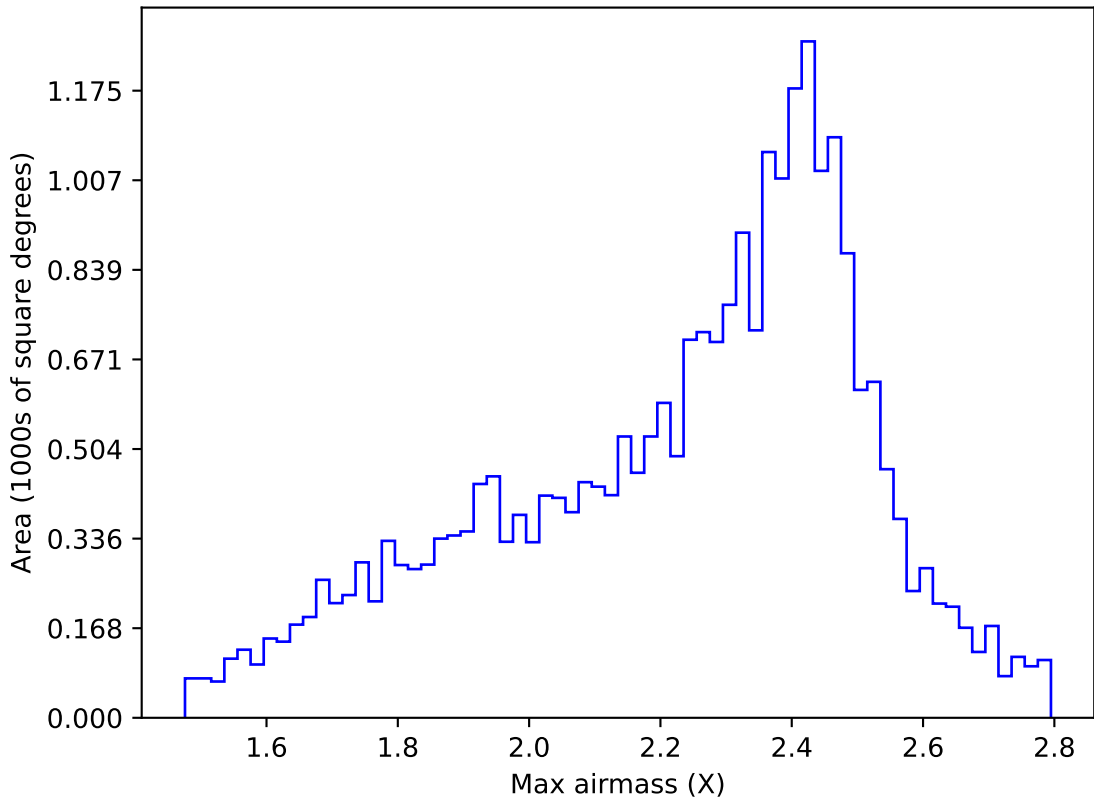
internal_u_expt60_nscale1.0v3.4_10yrs All sky r band: Max airmass
