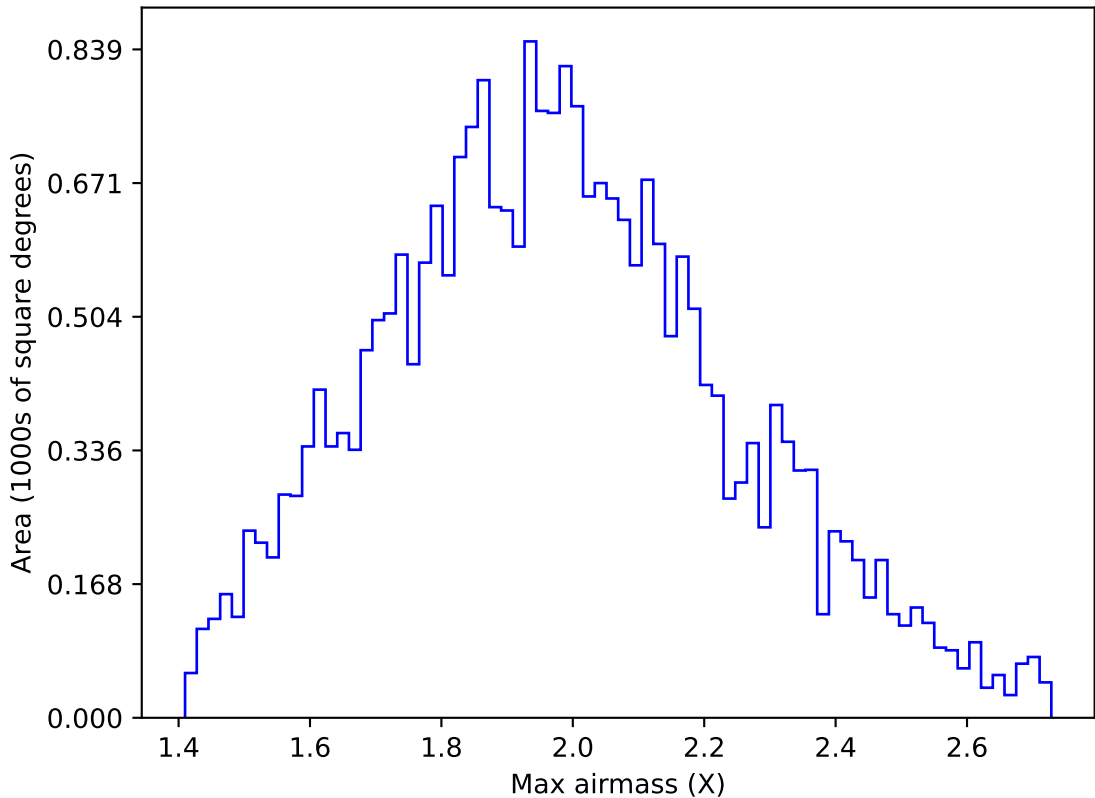
internal_u_expt60_nscale1.0v3.4_10yrs All sky g band: Max airmass
