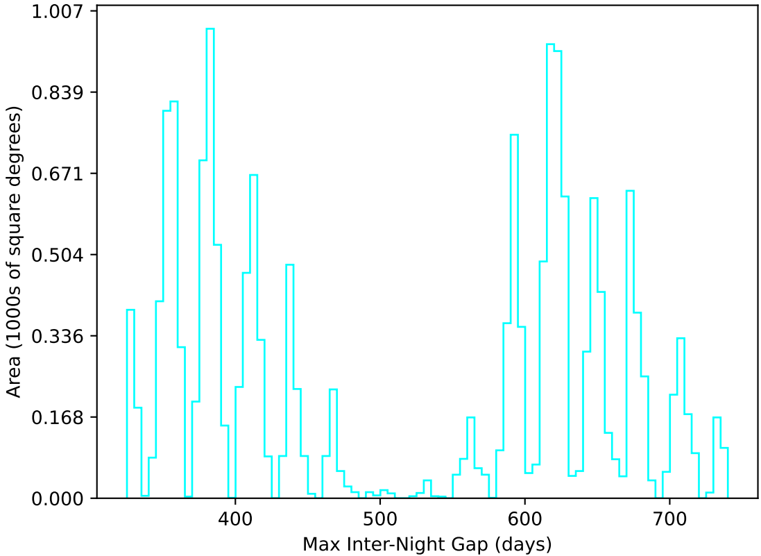
internal_u_expt60_nscale1.0v3.4_10yrs WFD u band: Max Inter-Night Gap
