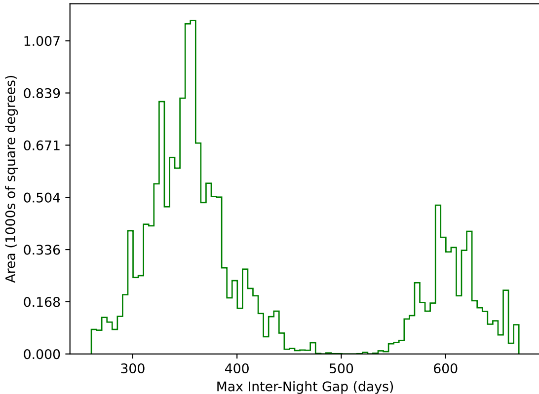
internal_u_expt60_nscale1.0v3.4_10yrs WFD g band: Max Inter-Night Gap
