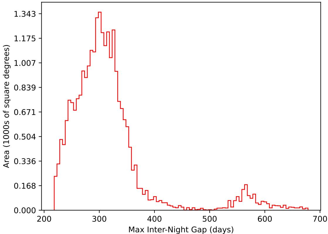
internal_u_expt60_nscale1.0v3.4_10yrs All sky i band: Max Inter-Night Gap
