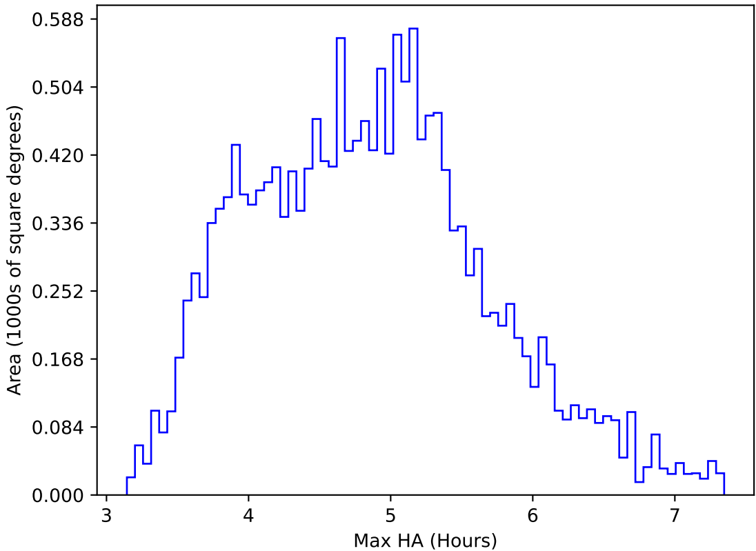
internal_u_expt60_nscale1.0v3.4_10yrs WFD i band: Max HA
