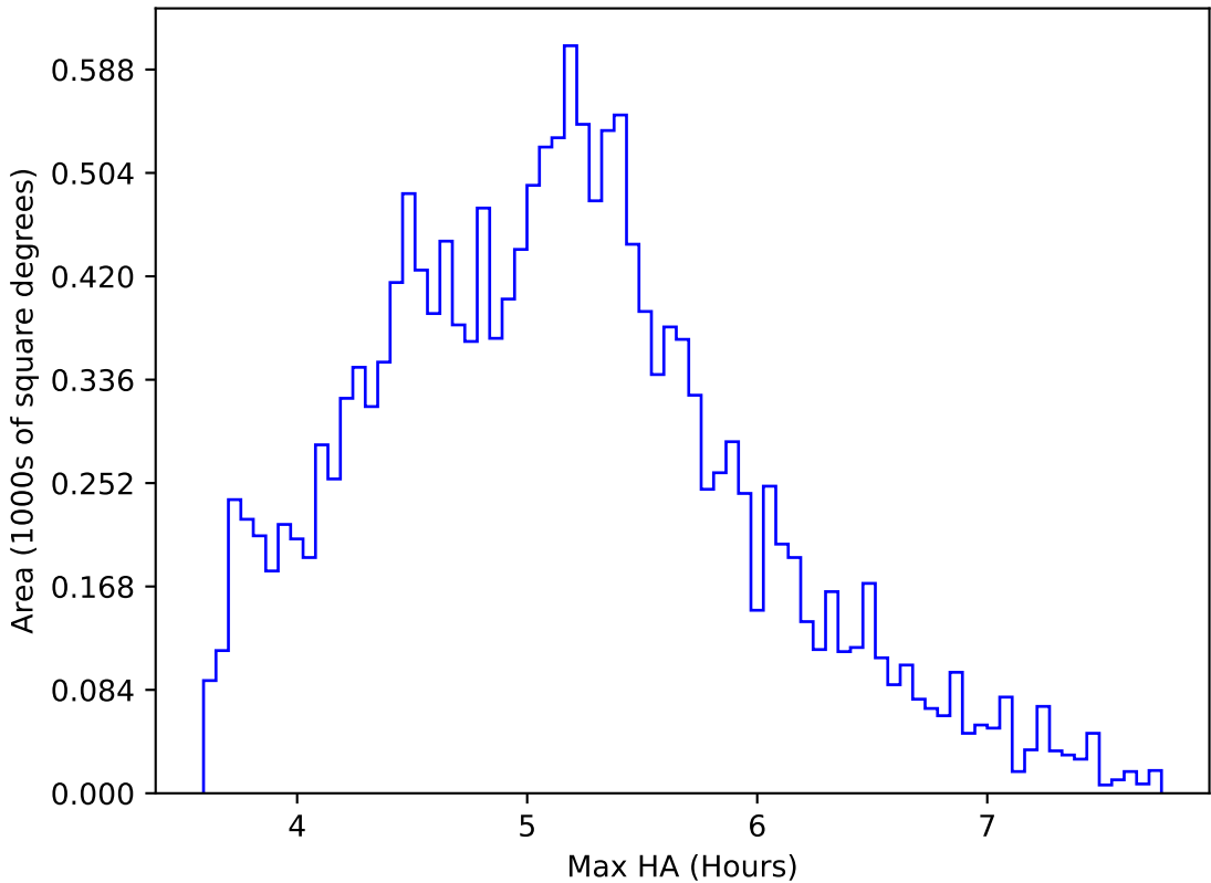
internal_u_expt60_nscale1.0v3.4_10yrs WFD all bands: Max HA
