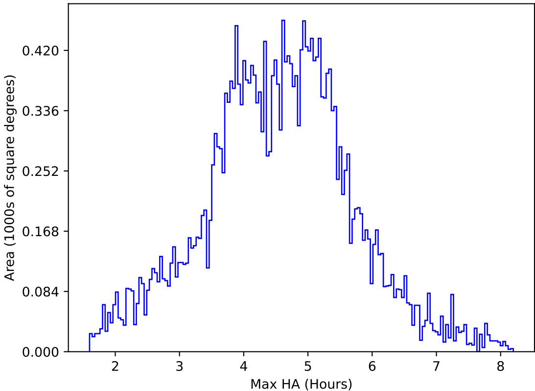
internal_u_expt60_nscale1.0v3.4_10yrs All sky i band: Max HA
