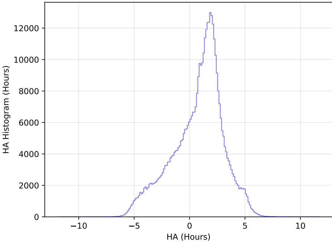
internal_u_expt60_nscale1.0v3.4_10yrs WFD z band: HA Histogram
