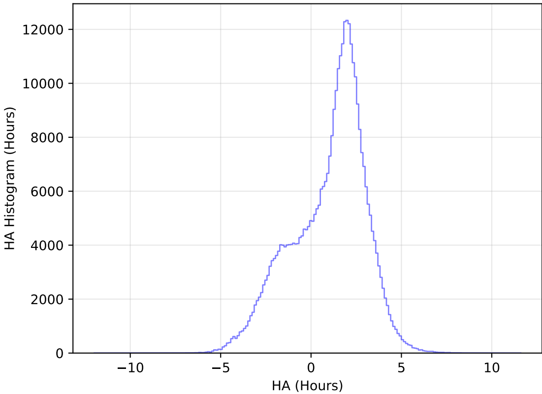
internal_u_expt60_nscale1.0v3.4_10yrs WFD y band: HA Histogram
