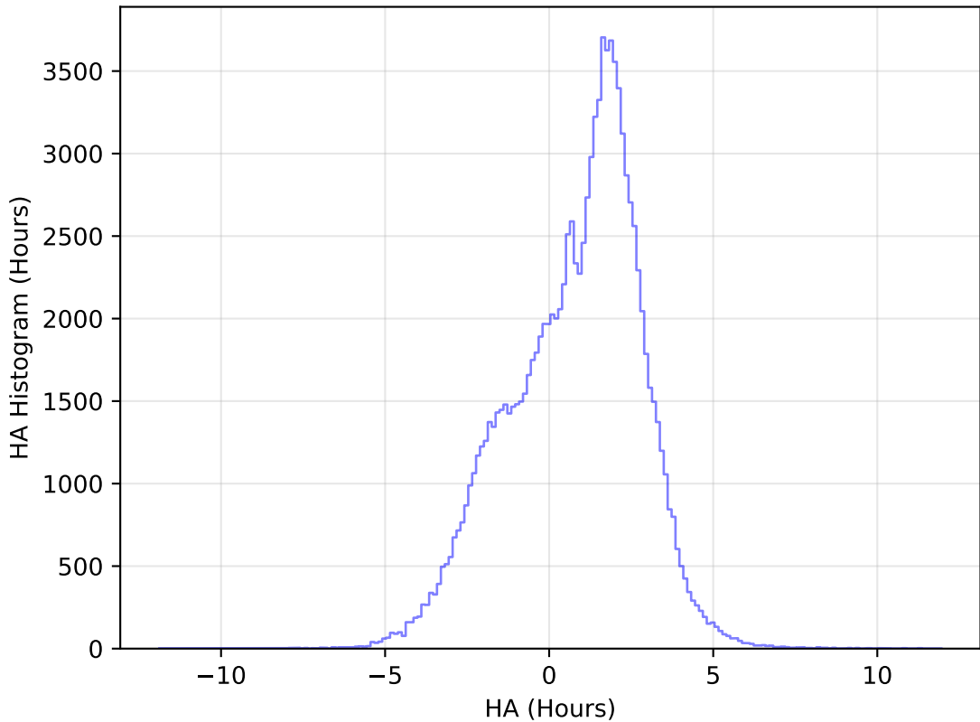
internal_u_expt60_nscale1.0v3.4_10yrs WFD u band: HA Histogram
