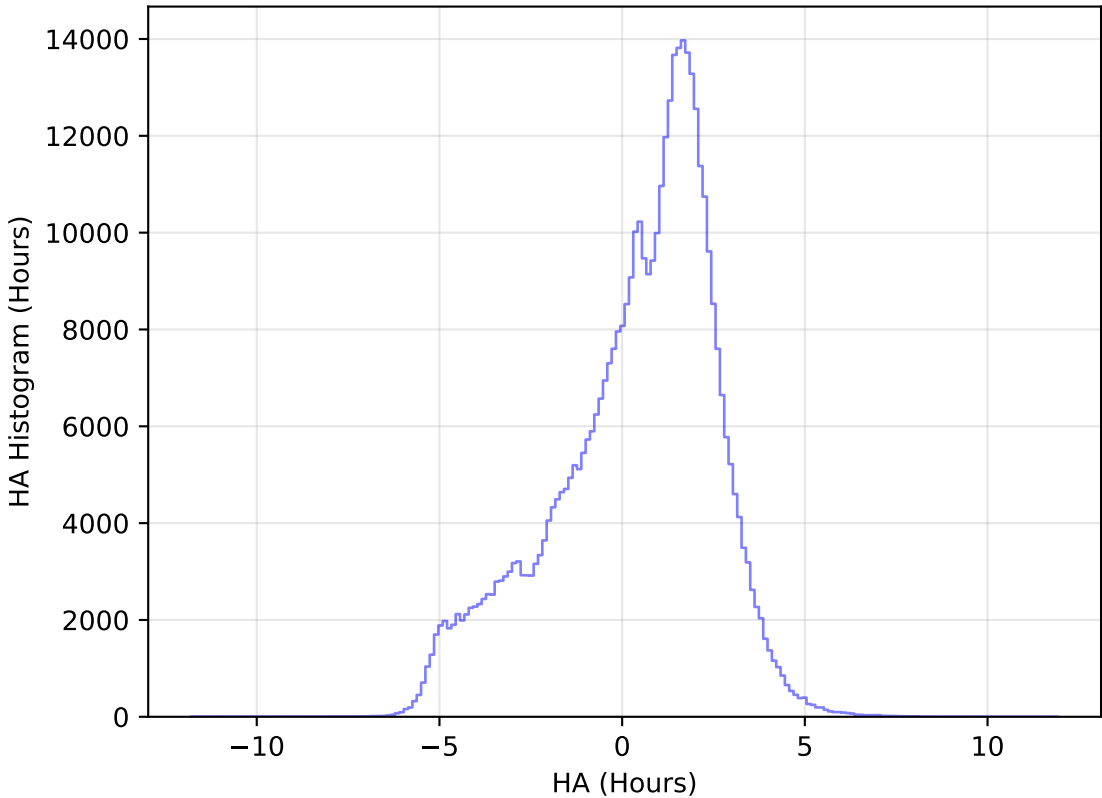
internal_u_expt60_nscale1.0v3.4_10yrs WFD r band: HA Histogram
