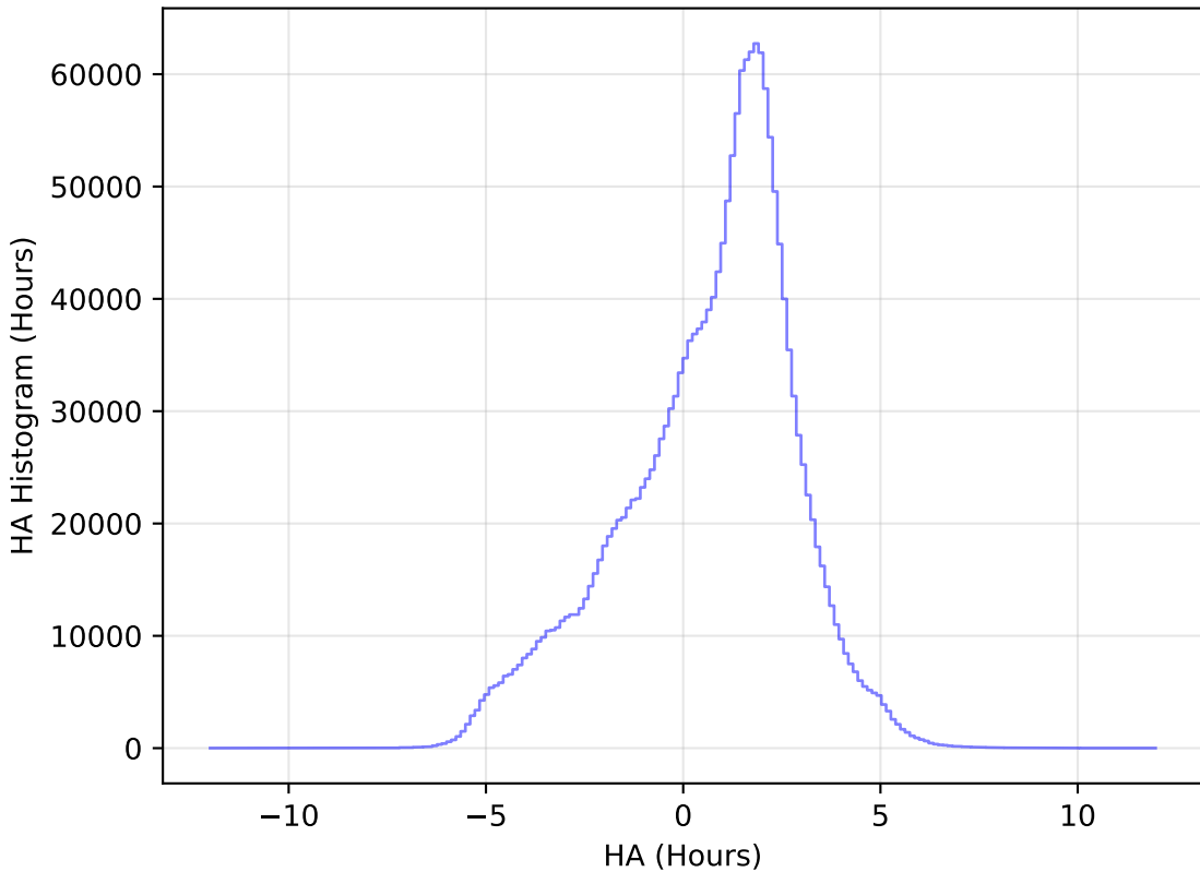
internal_u_expt60_nscale1.0v3.4_10yrs WFD all bands: HA Histogram
