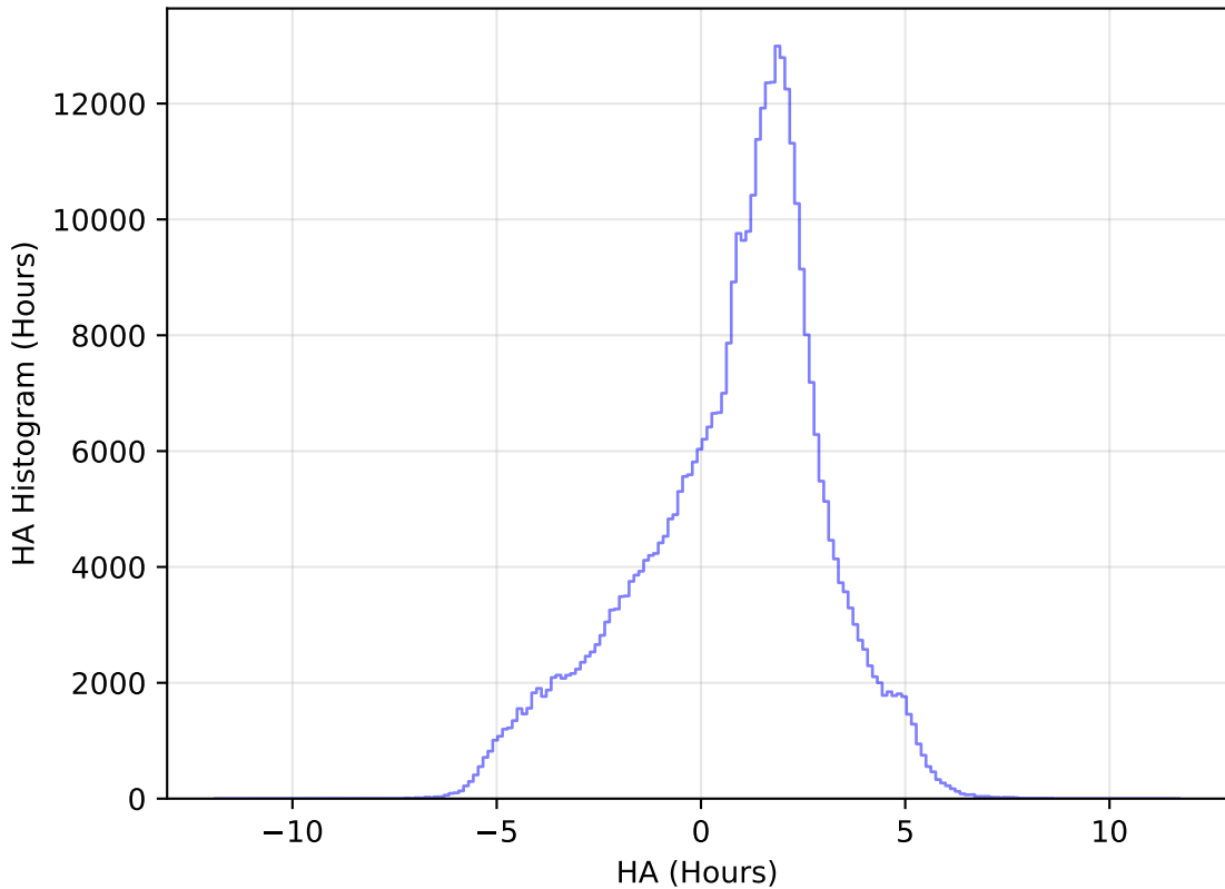
internal_u_expt60_nscale1.0v3.4_10yrs All sky z band: HA Histogram
