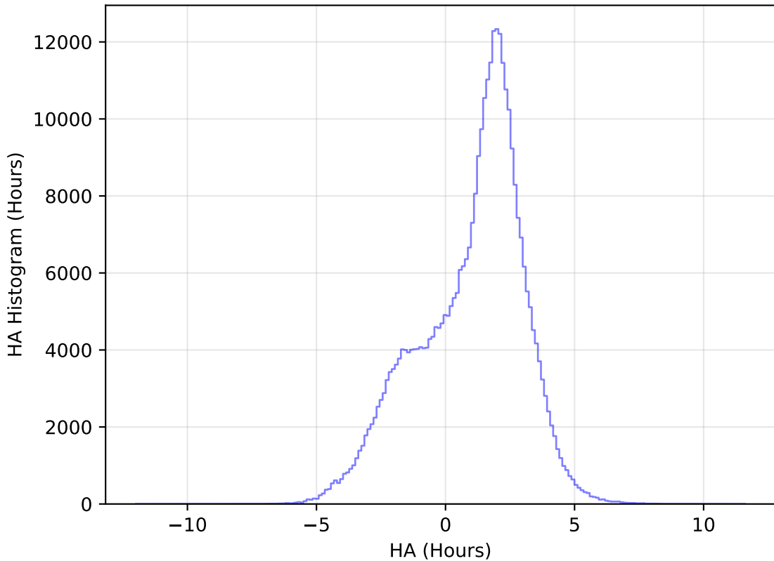
internal_u_expt60_nscale1.0v3.4_10yrs All sky y band: HA Histogram
