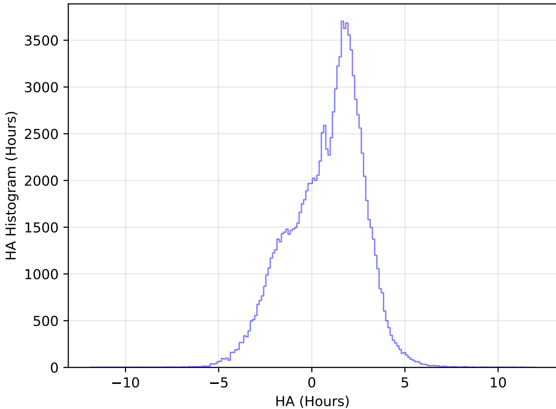
internal_u_expt60_nscale1.0v3.4_10yrs All sky u band: HA Histogram
