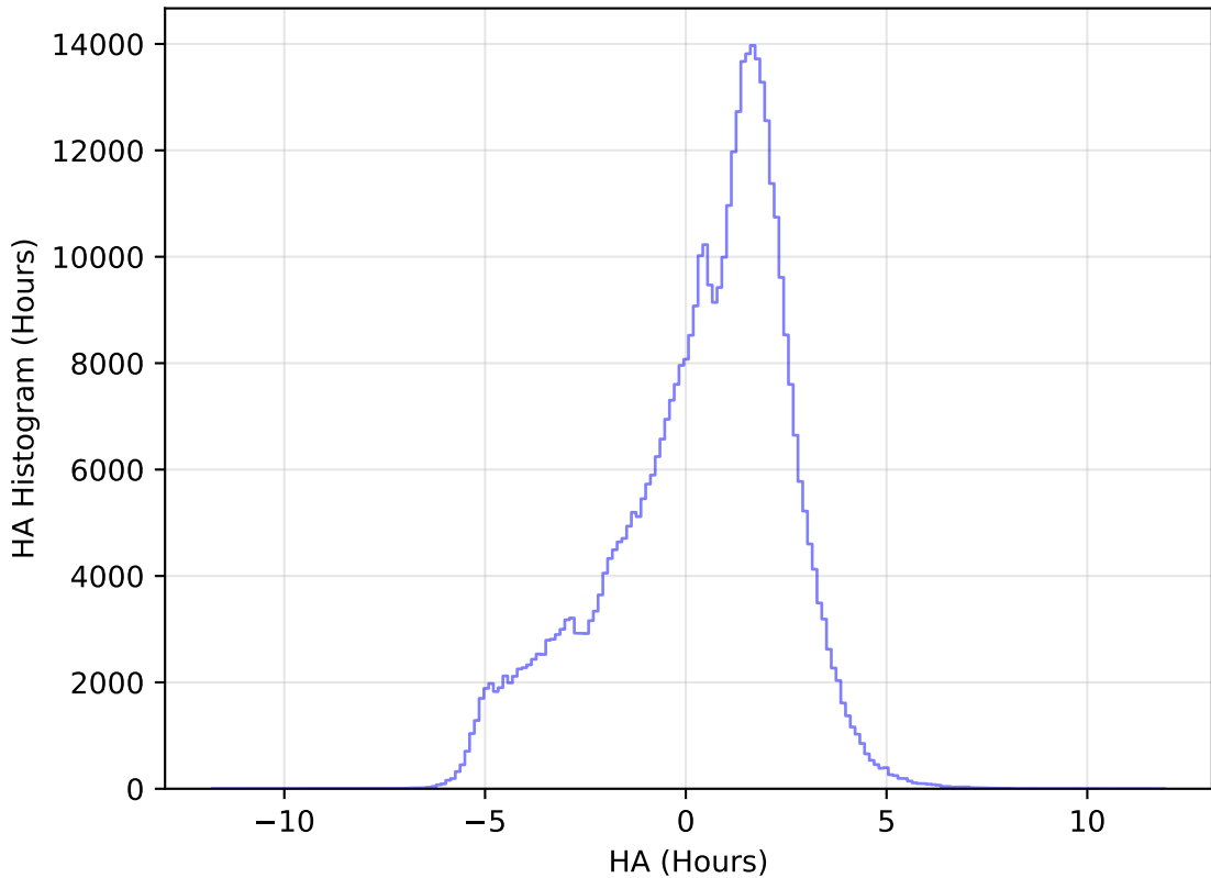
internal_u_expt60_nscale1.0v3.4_10yrs All sky r band: HA Histogram
