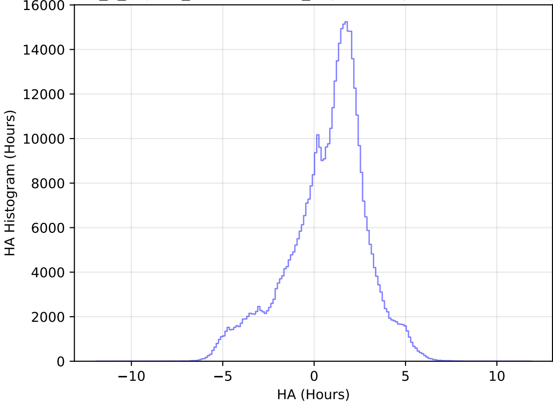
internal_u_expt60_nscale1.0v3.4_10yrs All sky i band: HA Histogram
