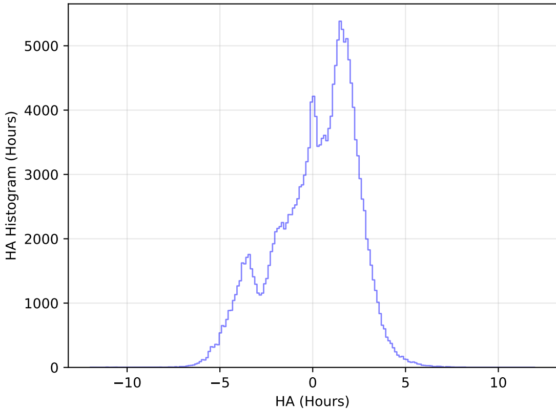
internal_u_expt60_nscale1.0v3.4_10yrs All sky g band: HA Histogram
