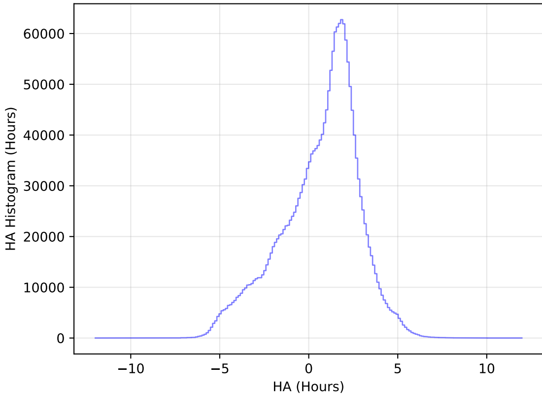
internal_u_expt60_nscale1.0v3.4_10yrs All sky all bands: HA Histogram
