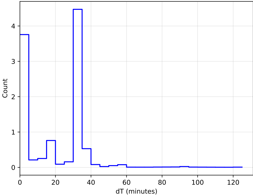
internal_u_expt60_nscale1.0v3.4_10yrs WFD: DeltaT Histogram
