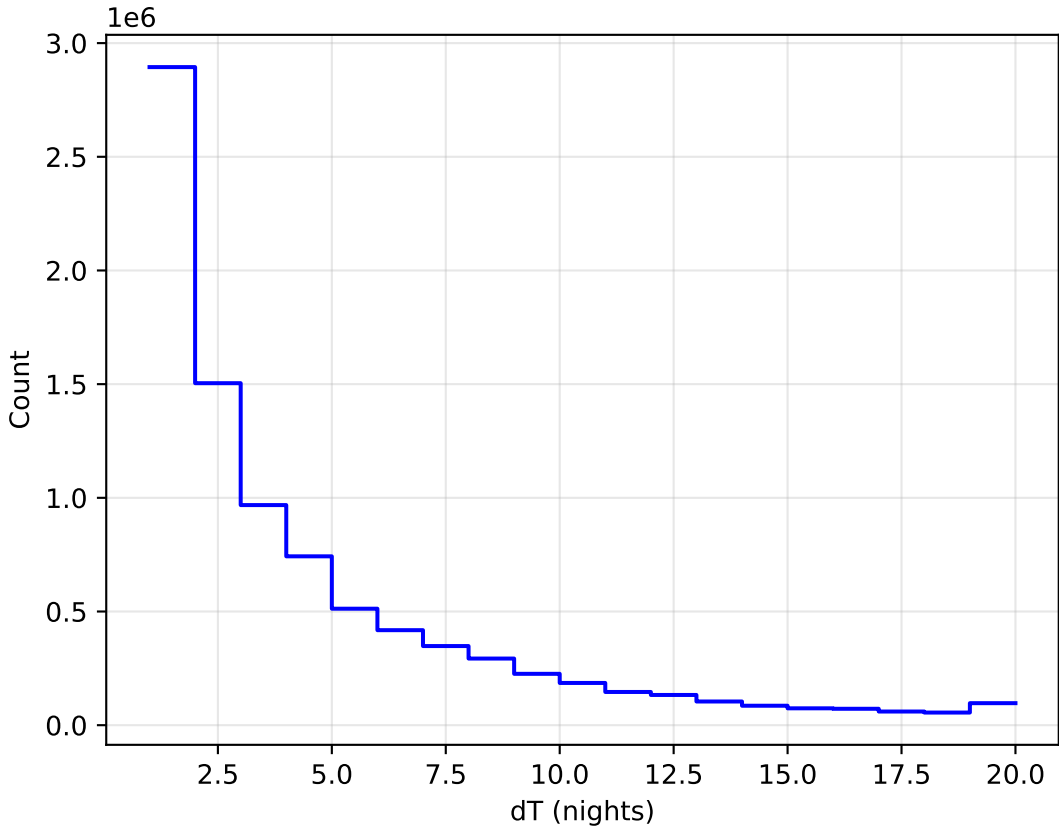
internal_u_expt60_nscale1.0v3.4_10yrs All sky all bands: DeltaNight Histogram
