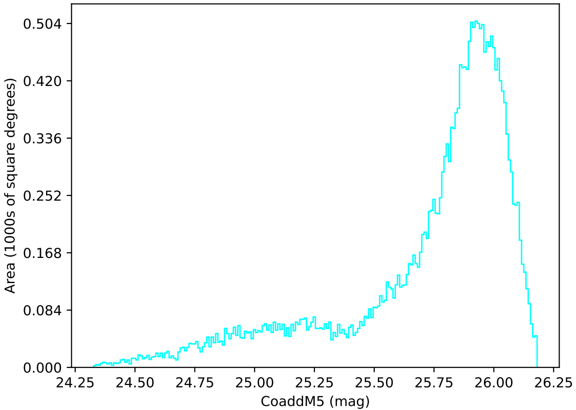
internal_u_expt60_nscale1.0v3.4_10yrs All sky u band: CoaddM5
