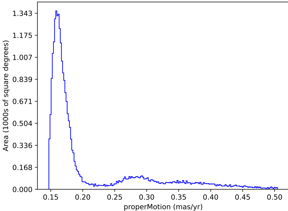
internal_u_expt60_nscale1.0v3.4_10yrs : properMotion
