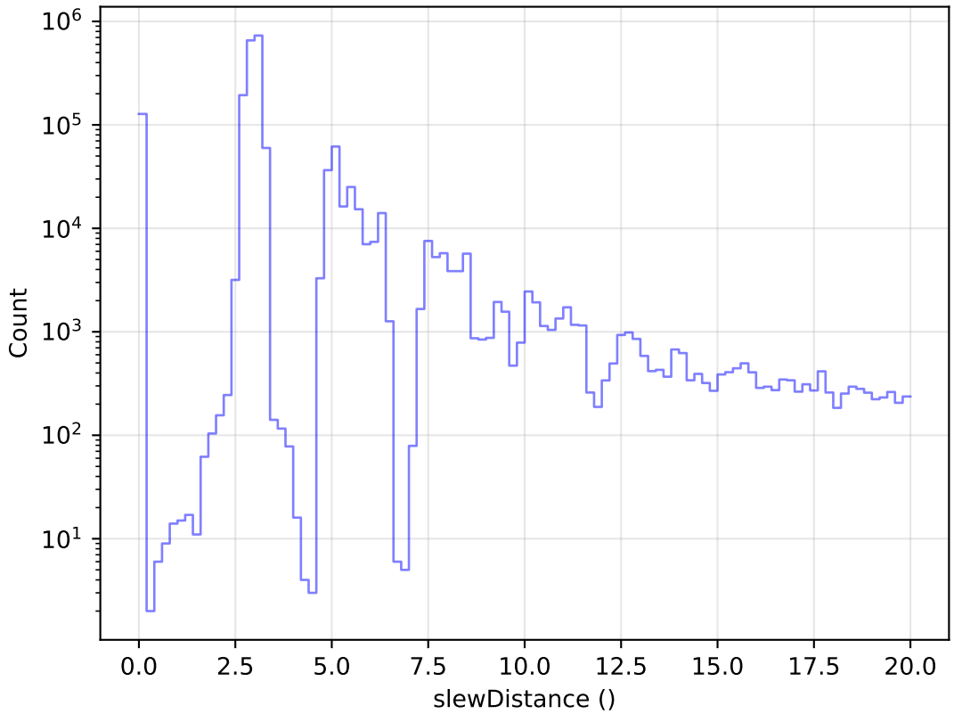
internal_u_expt60_nscale1.0v3.4_10yrs All visits: Zoom Slew Distance Histogram
