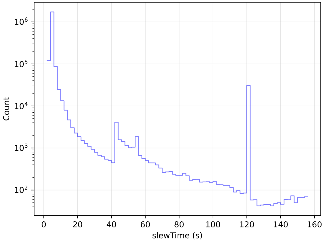
internal_u_expt60_nscale1.0v3.4_10yrs All visits: Slew Time Histogram
