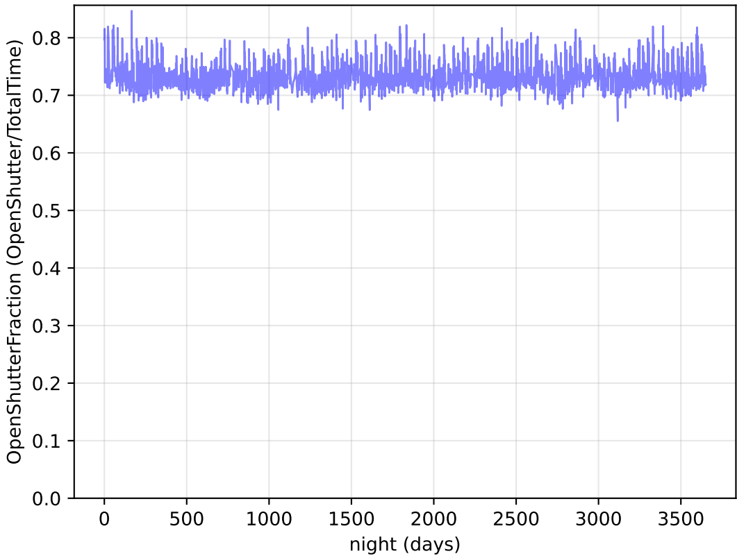
internal_u_expt60_nscale1.0v3.4_10yrs : OpenShutterFraction
