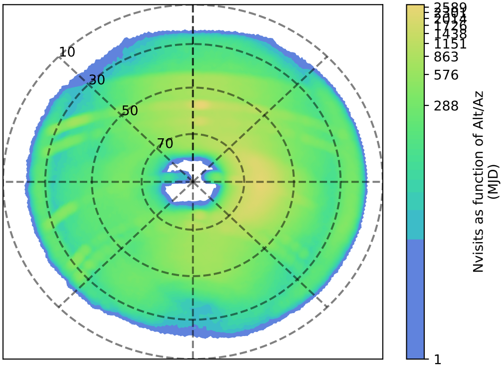
internal_u_expt60_nscale1.0v3.4_10yrs i: Nvisits as function of Alt/Az
