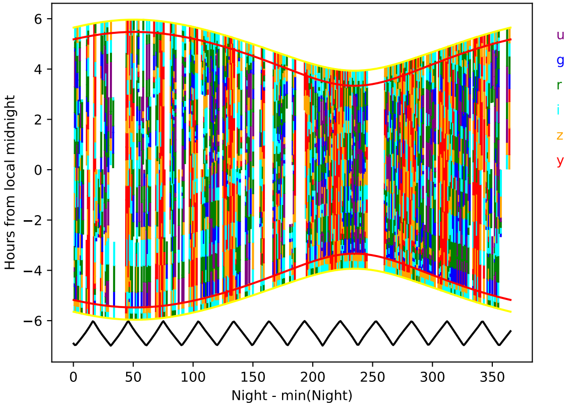
internal_u_expt60_nscale1.0v3.4_10yrs year 5-6: Hourglass
